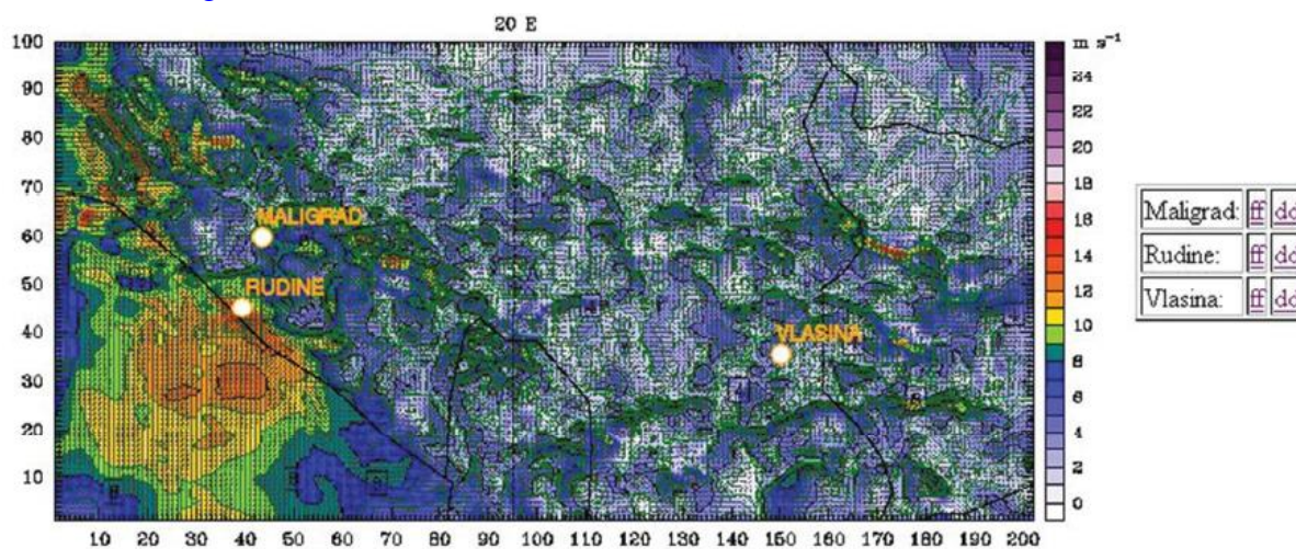
Fig. 12: Picture 4; Wind forecast based on WRF model
