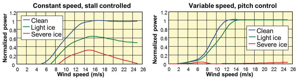
Figure 7-2: The impact ice on the power curves of stall (left) and pitch (right) regulated wind turbines in different icing conditions. Graph source: VTT Finland [12].
