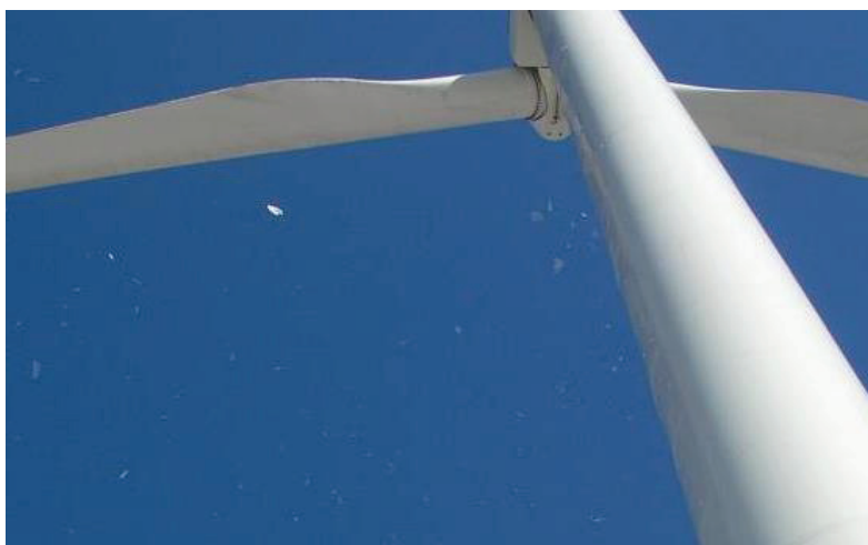
Figure 8-1: Ice falling or being thrown off a wind turbine poses a safety threat to turbine maintenance staff and, depending on turbine siting, the general public. Photo credit: Jeroen Van Dam, USA
