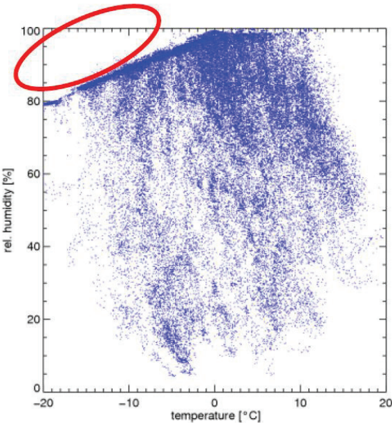
Figure 4-4: Relative humidity measured according WMO/CIMO standards does not reach saturation anymore at temperatures below 0°C (red area).
