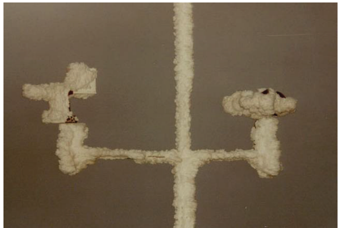
Figure 4-2: The impact of ice build-up on mounting hardware and sensors must be considered to ensure the accuracy of wind speed and direction measurements. Photo credit: Michael Durstewitz.
