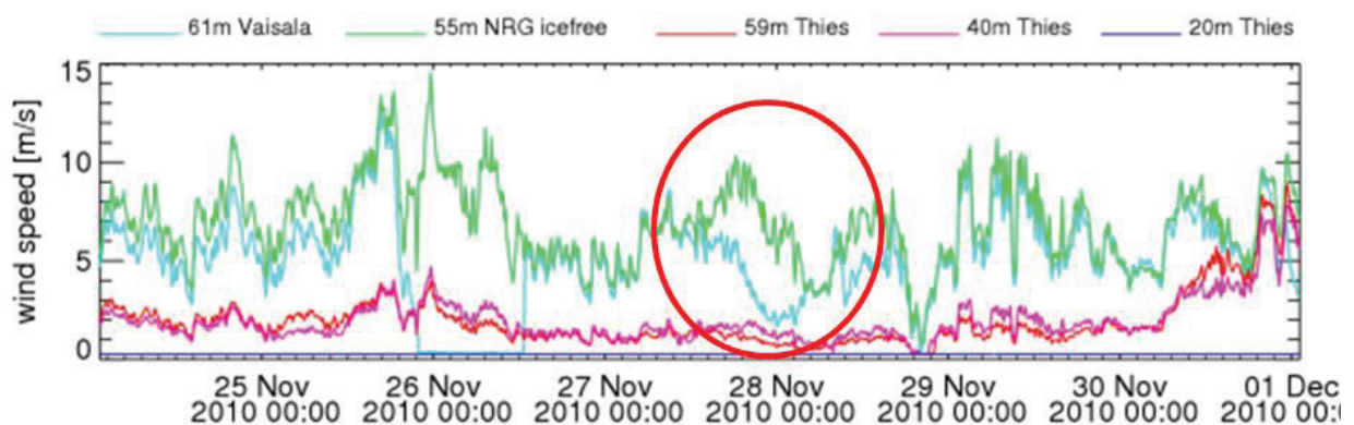
Figure 4-3: Comparison of two fully heated (green, cyan), two shaft heated (red and purple) and a fully unheated (blue, stand still) anemometer during an icing event.
